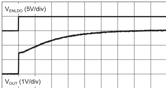
LDO Initial Power-Up Response Time
