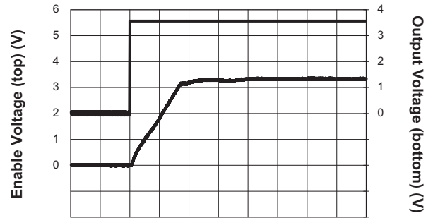
LDO Turn-On Time from Enable
