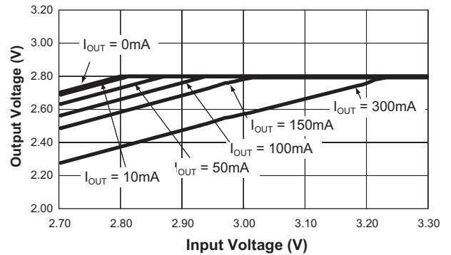
LDO Dropout Characteristics ( EN = \text{GND} ; ENLDO = V_{IN} )
