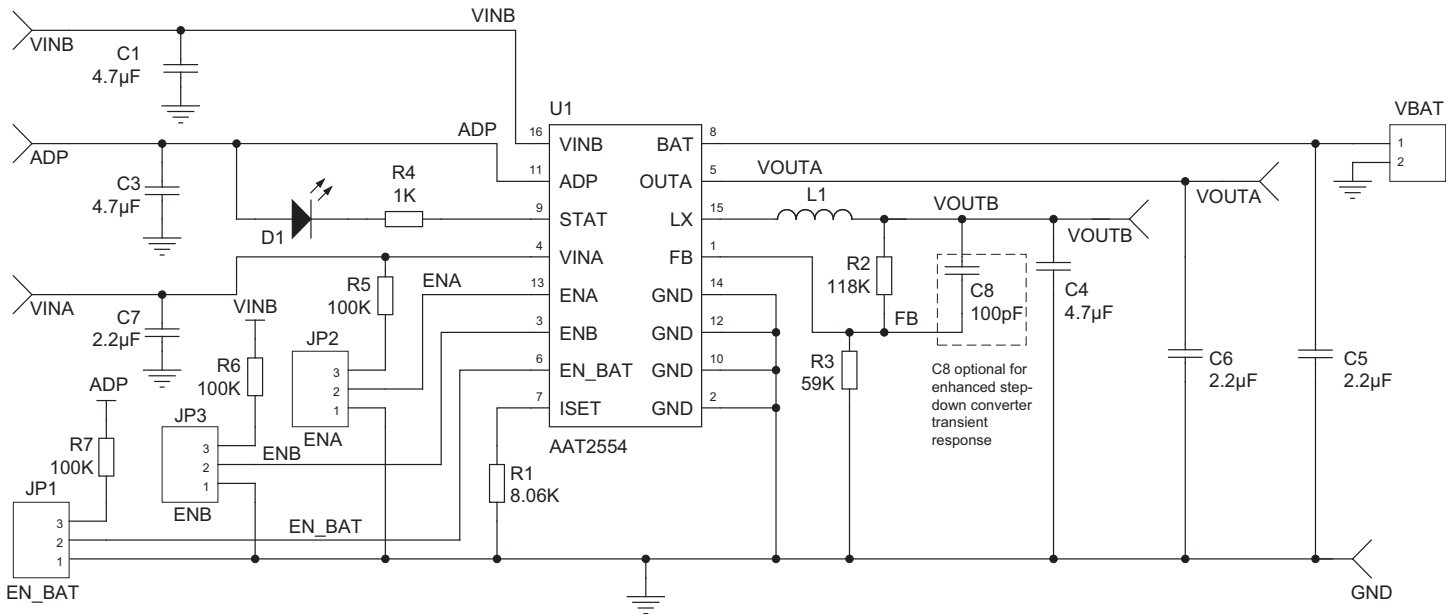
Figure 5: AAT2554 Evaluation Board Schematic.
