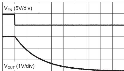
Turn-Off Response Time
