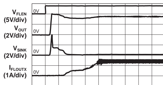
Flash Turn On Characteristic ( I_{FLOUTX} = 750\text{mA/ch} ; V_{IN} = 3.6\text{V} ; L = 1\mu\text{H} )
