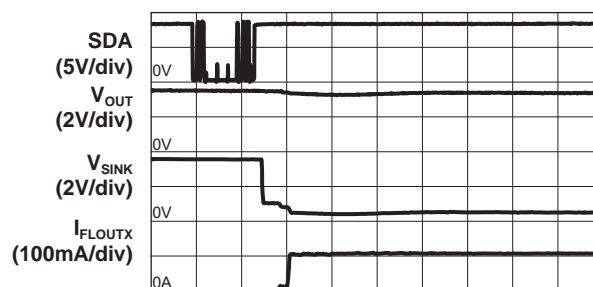
Movie Mode Turn On Characteristic ( I_{FLOUTX} = 103\text{mA/ch} ; V_{IN} = 3.6\text{V} ; L = 1\mu\text{H} )
