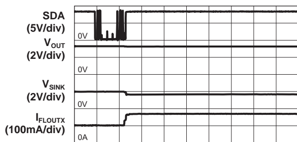
Movie Mode Transition Characteristic ( I_{FLOUTX} = 102\text{mA to } 188\text{mA/ch} ; C_{OUT} = 0.22\mu\text{F} ; V_{IN} = 3.6\text{V} ; L = 1\mu\text{H} )
