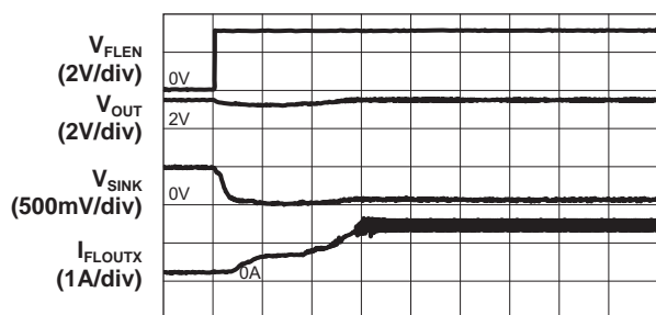
Movie Mode to Flash Turn On Characteristic ( I_{FLOUTX} = 103\text{mA to } 750\text{mA/ch} ; V_{IN} = 3.6\text{V} ; L = 1\mu\text{H} )
