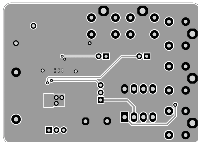
Figure 5: AAT1271 Evaluation Board Bottom Side Layout.
