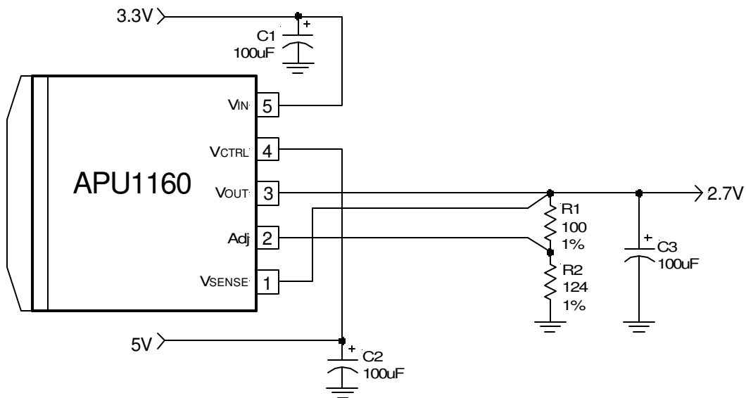
Figure 1 - Typical application of APU1160 in a 3.3V to 2.8V.
