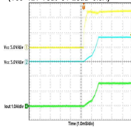
Power-ON (Vcc=12V Vout=9V Load=0.8A)
