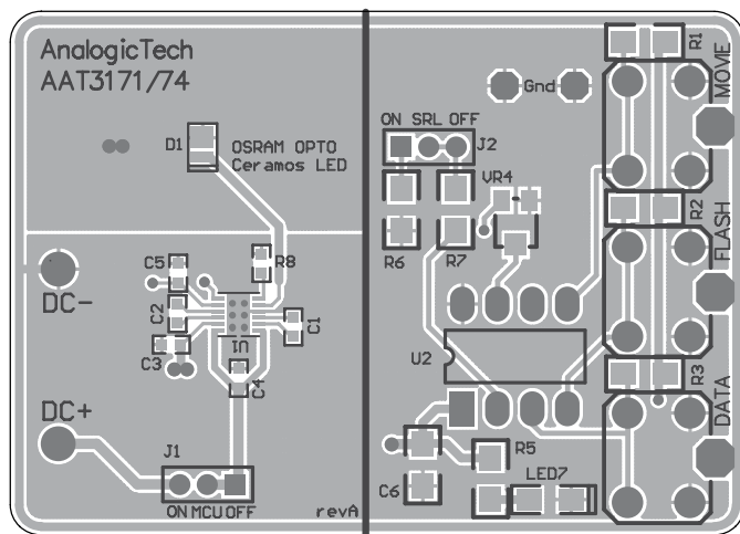
Figure 5: AAT3171 Evaluation Board Top Side Layout.
