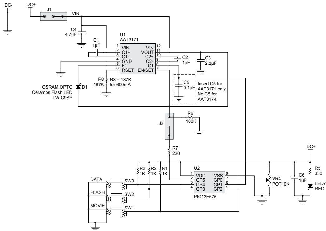
Figure 7: AAT3171 Evaluation Board Schematic.
