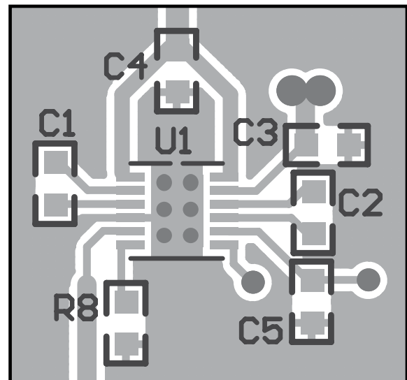
Figure 4: Example PCB Layout.
