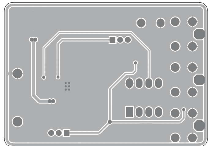
Figure 6: AAT3171 Evaluation Board Bottom Side Layout.
