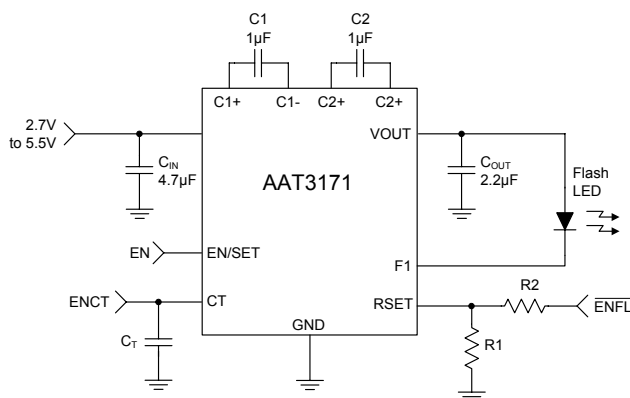
Figure 3: Flash/Torch Control Using the RSET Pin.
