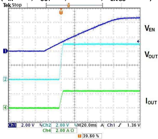
Enable-ON Wave (60KHz) ( V_{IN}=12V , V_{OUT}=5V , Load=2A, C_{EN/SS}=0.1\mu F )
