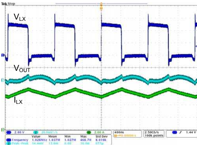
Fig.11 Output Ripple, Vin=5V, Vo=1.8V, Io=6A
