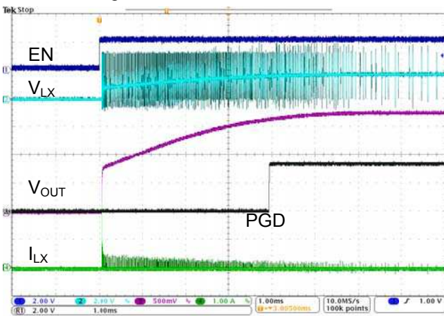
Fig.1 Enable, 5Vi to 1.8Vo/0A
