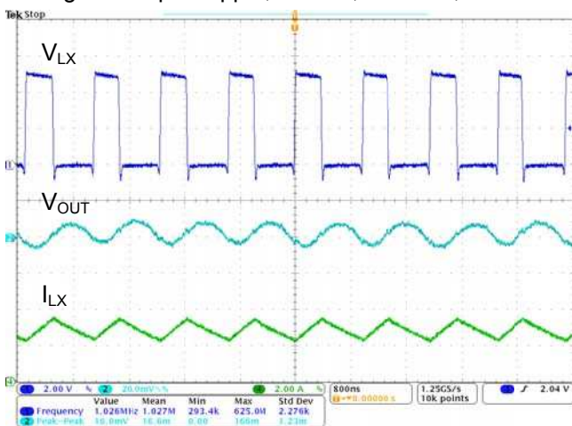
Fig.11 Output Ripple, Vin=5V, Vo=1.8V, Io=3A
