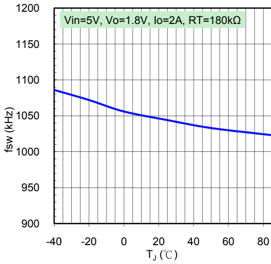
Fig.19 Switching Frequency vs. Temperature
