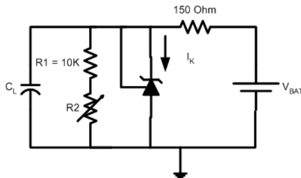
Test Circuit for V_{KA} = 2\text{V}, 3\text{V}
