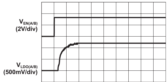
Time (40µs/div)
