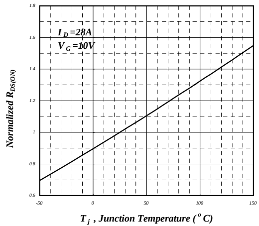
Fig 4. Normalized On-Resistance
