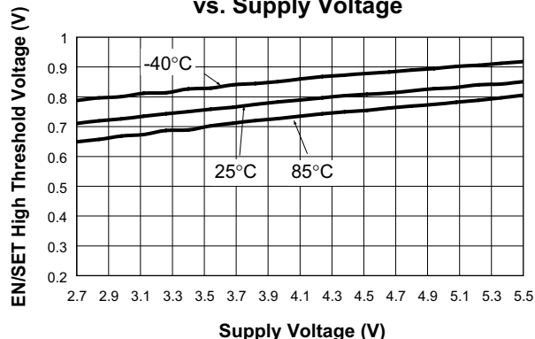
EN/SET High Threshold Voltage vs. Supply Voltage
