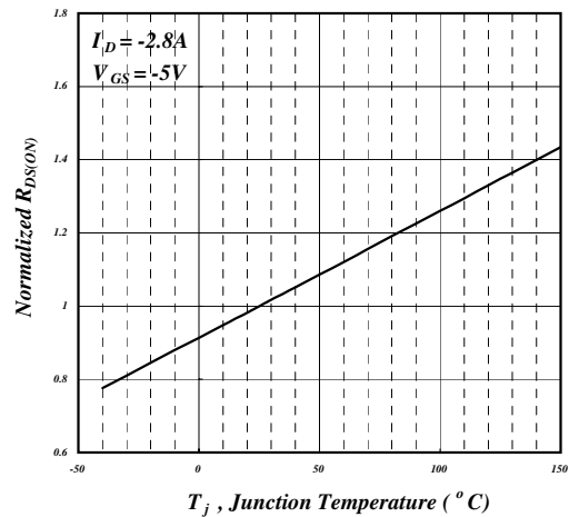
Fig 4. Normalized On-Resistance
