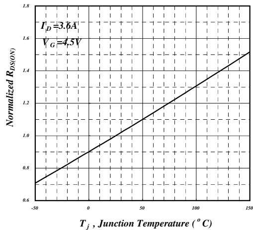
Fig 4. Normalized On-Resistance
