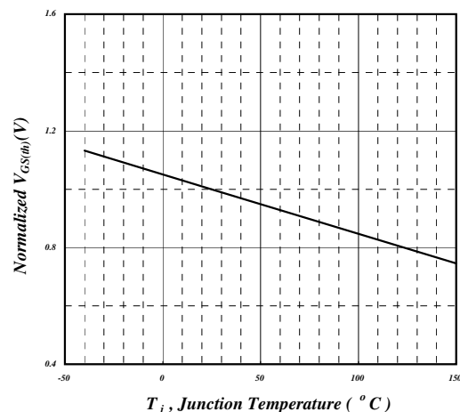
Fig 6. Normalized Gate Threshold Voltage v.s. Junction Temperature
