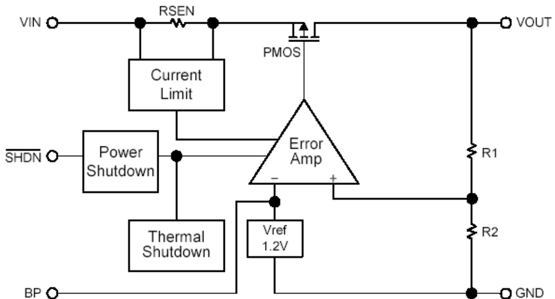
Figure 2. Block Diagram of APE8800A
