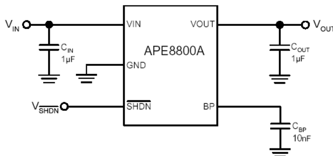
Figure 1. Typical Application Circuit of APE8800A
