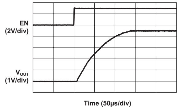
Startup Time with 200mA Load
