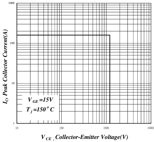
Fig 7. Reverb Bias SOA
