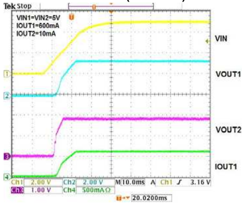
Power ON Test (Channel 1)
