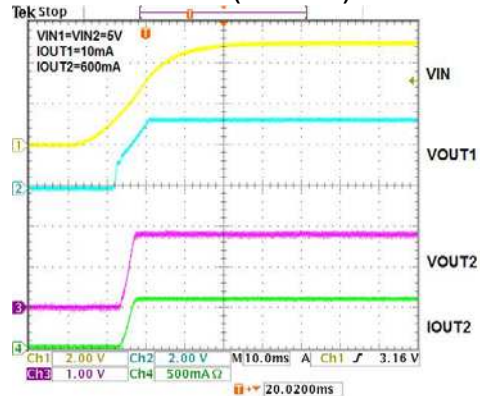
Power ON Test (Channel 2)
