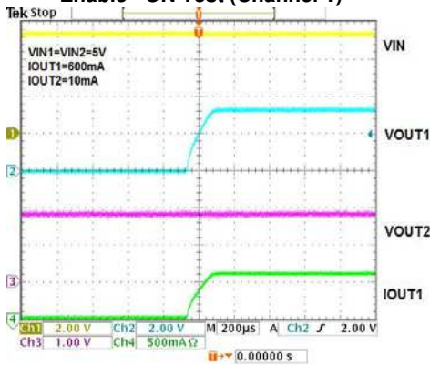
Enable -ON Test (Channel 1)
