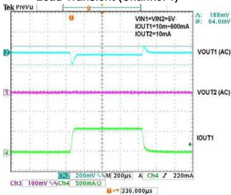
Load Transient (Channel 1)
