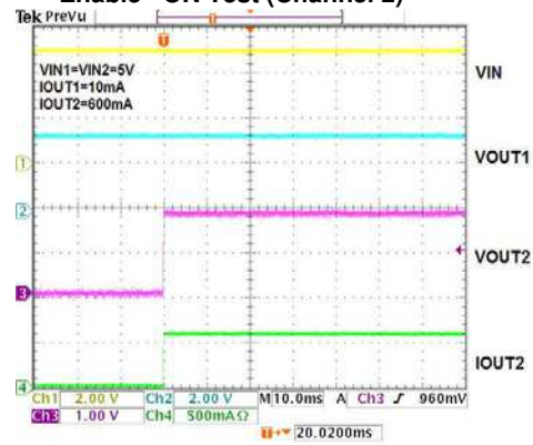
Enable -ON Test (Channel 2)
