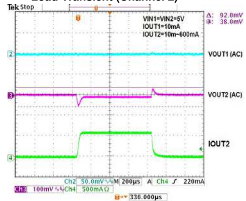
Load Transient (Channel 2)
