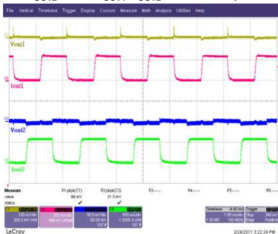
Load Transient ( V_{IN1}=V_{IN2}=5V , V_{OUT1}=3.3V , V_{OUT2}=1.2V , I_{OUT1}=I_{OUT2}=10\sim 600mA )
