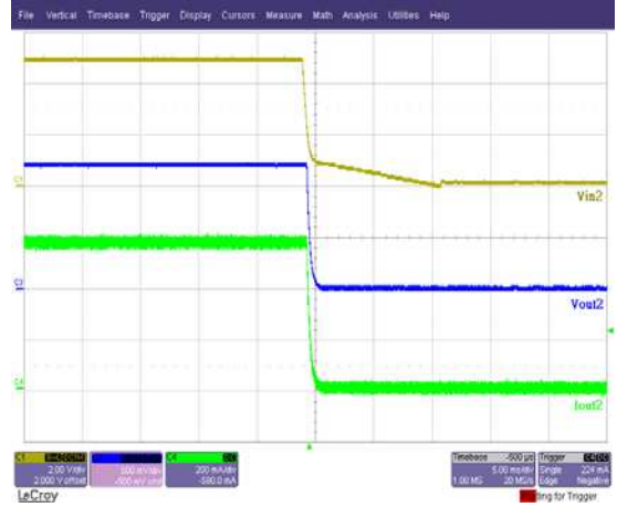
Power Off (Channel-2)
