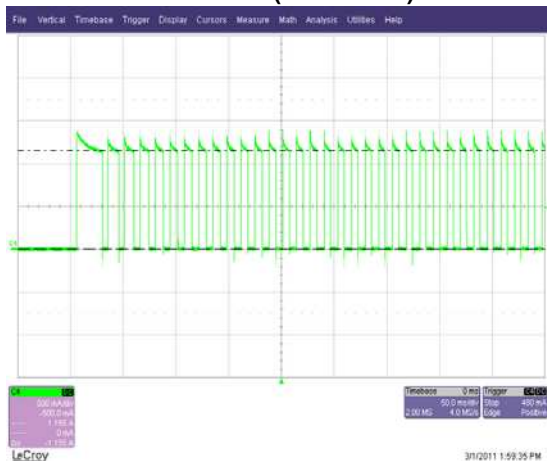
Current Limit (Channel-1)
