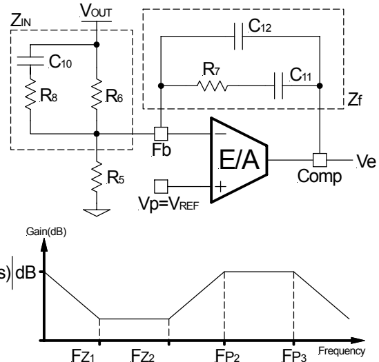
Figure 16- Compensation network with local feedback and its asymptotic gain plot.
