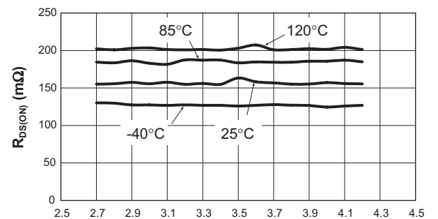
Load Switch R_{DS(ON)} vs. Input Voltage
