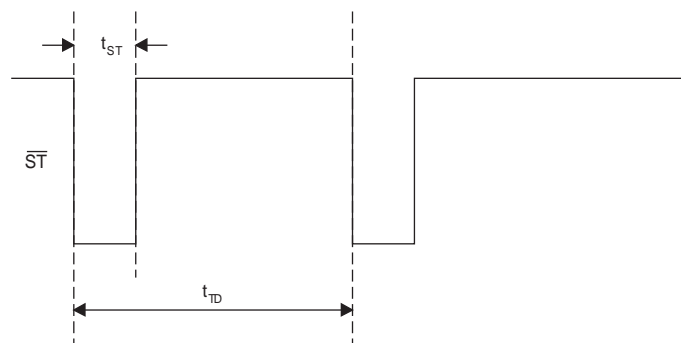
Figure 3: Watchdog Input.
