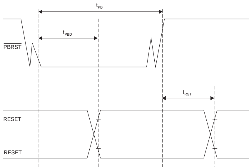
Figure 2: Push-Button Reset.
