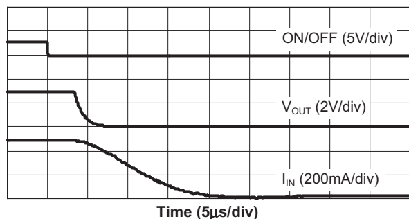
AAT4280A-2 Turn-Off
