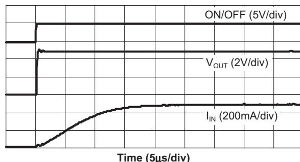
AAT4280A-2 Turn-On
