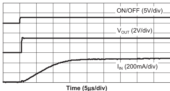
AAT4280A-2 Turn-On
