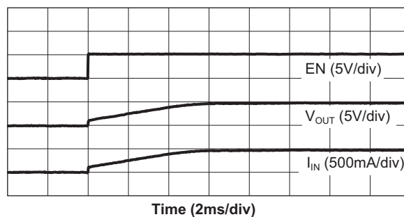
AAT4280A-4 Turn-On ( V_{IN} = 5V ; R_L = 10\Omega )
