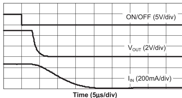
AAT4280A-2 Turn-Off
