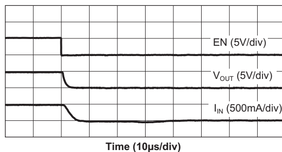
AAT4280A-4 Turn-Off ( V_{IN} = 5V ; R_L = 10\Omega )
