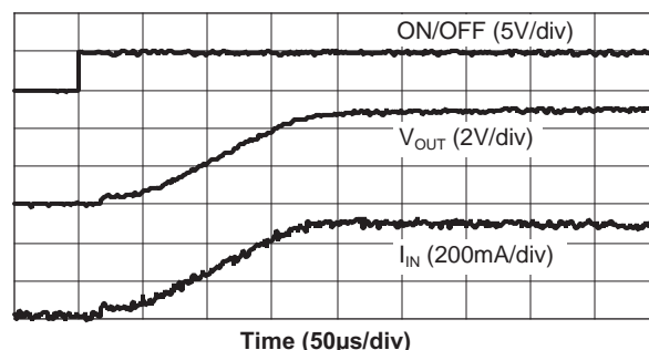
AAT4280-3 Turn-On
