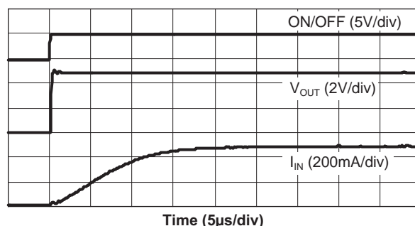
AAT4280-2 Turn-On
