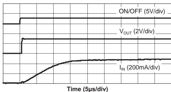
AAT4280-2 Turn-On
