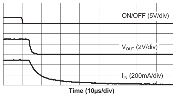
AAT4280-1 Turn-Off
