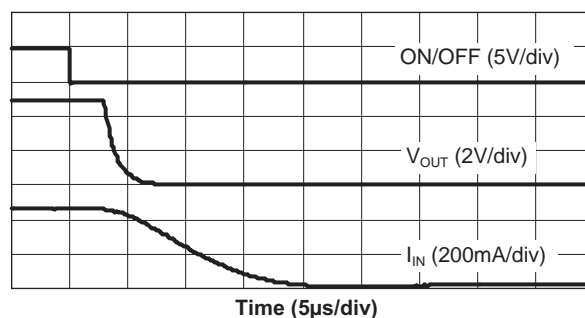
AAT4280-2 Turn-Off
