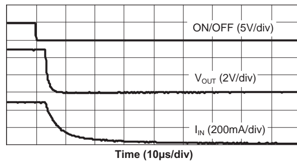
AAT4280-1 Turn-Off
