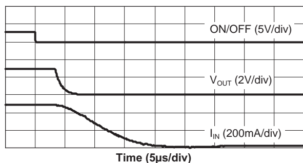
AAT4280-2 Turn-Off
