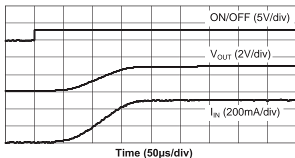
AAT4280-3 Turn-On
