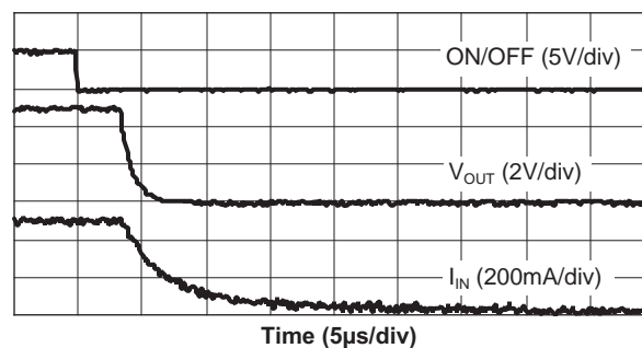
AAT4280-3 Turn-Off
