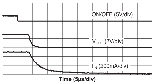
AAT4280-3 Turn-Off
