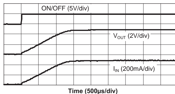
AAT4280-1 Turn-On
