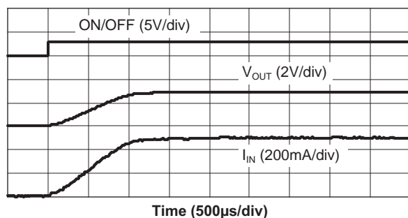
AAT4280-1 Turn-On
