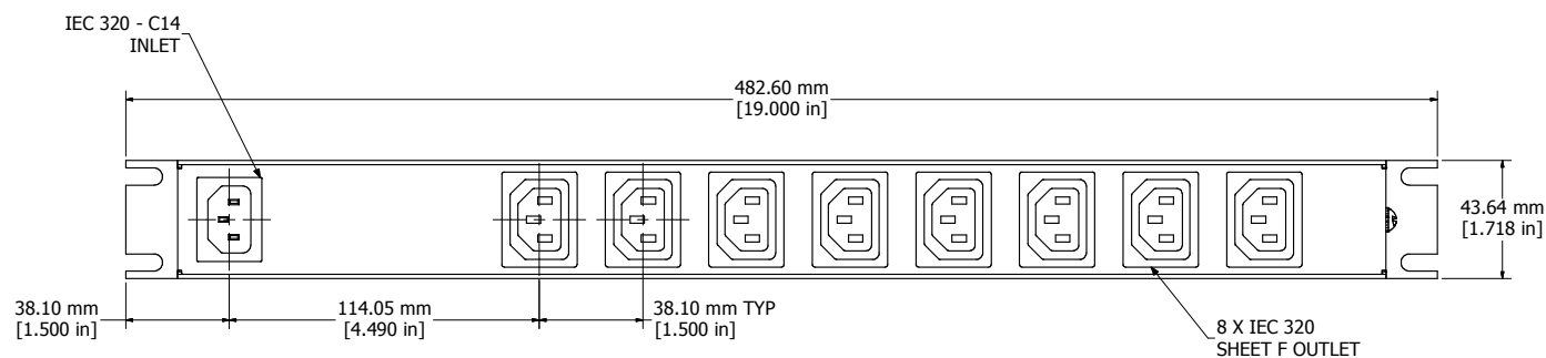
ASSEMBLY - VIEW FROM BACK
