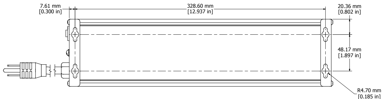
ASSEMBLY - VIEW FROM BOTTOM
