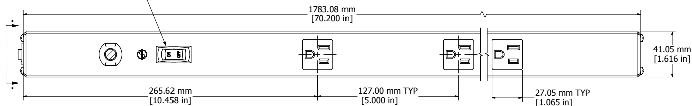
SECTION A-A (VIEW FROM FRONT)
