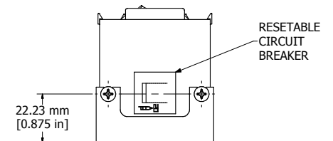
ASSEMBLY - VIEW FROM END
