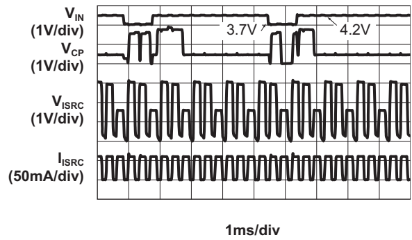
Line Response (1X Mode; I_{ISRC} = 60mA )
