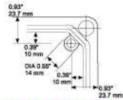
Typical Corner View Polyester Cover
