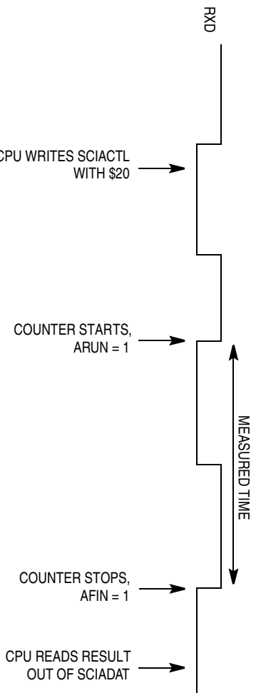
Figure 15-21. Bit Time Measurement with ACLK = 0
