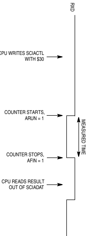
Figure 15-23. Bit Time Measurement with ACLK = 1, Scenario B
