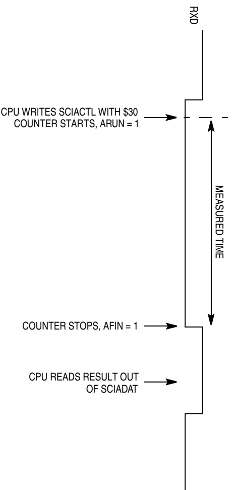
Figure 15-22. Bit Time Measurement with ACLK = 1, Scenario A
