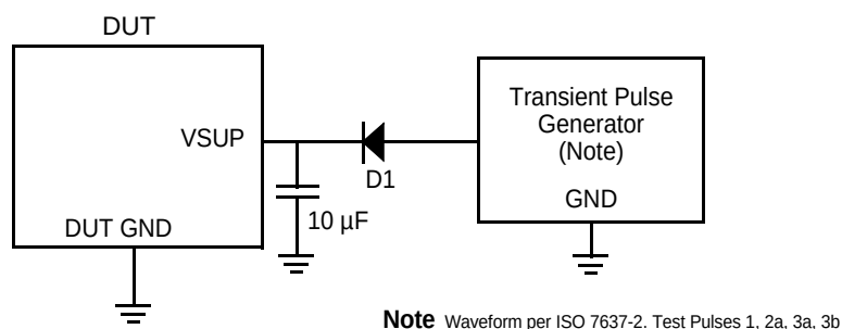
Figure 4. Test Circuit for Transient Test Pulses ( V_{SUP} )
