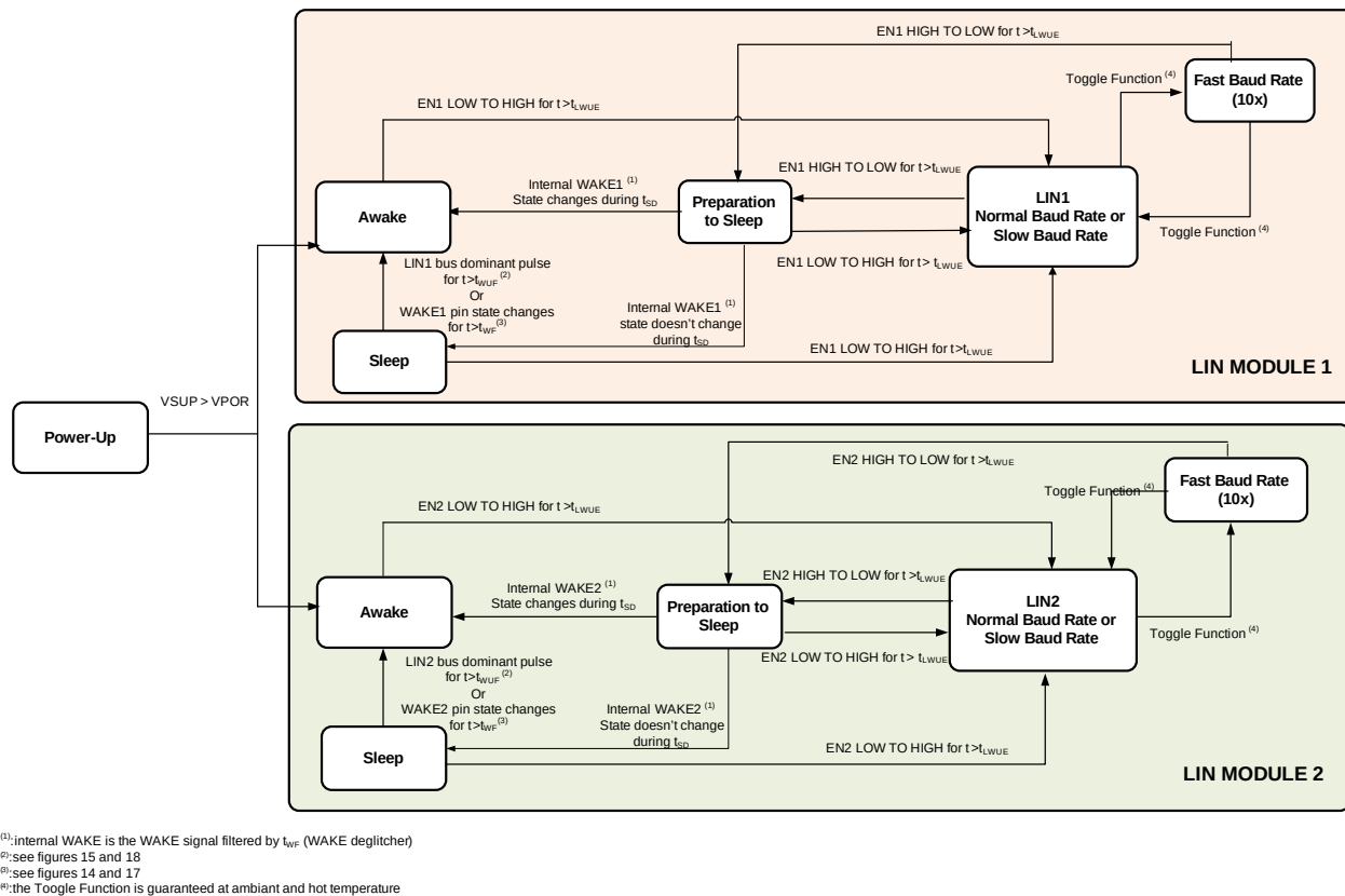
Figure 25. Operational and Transitional Modes State
