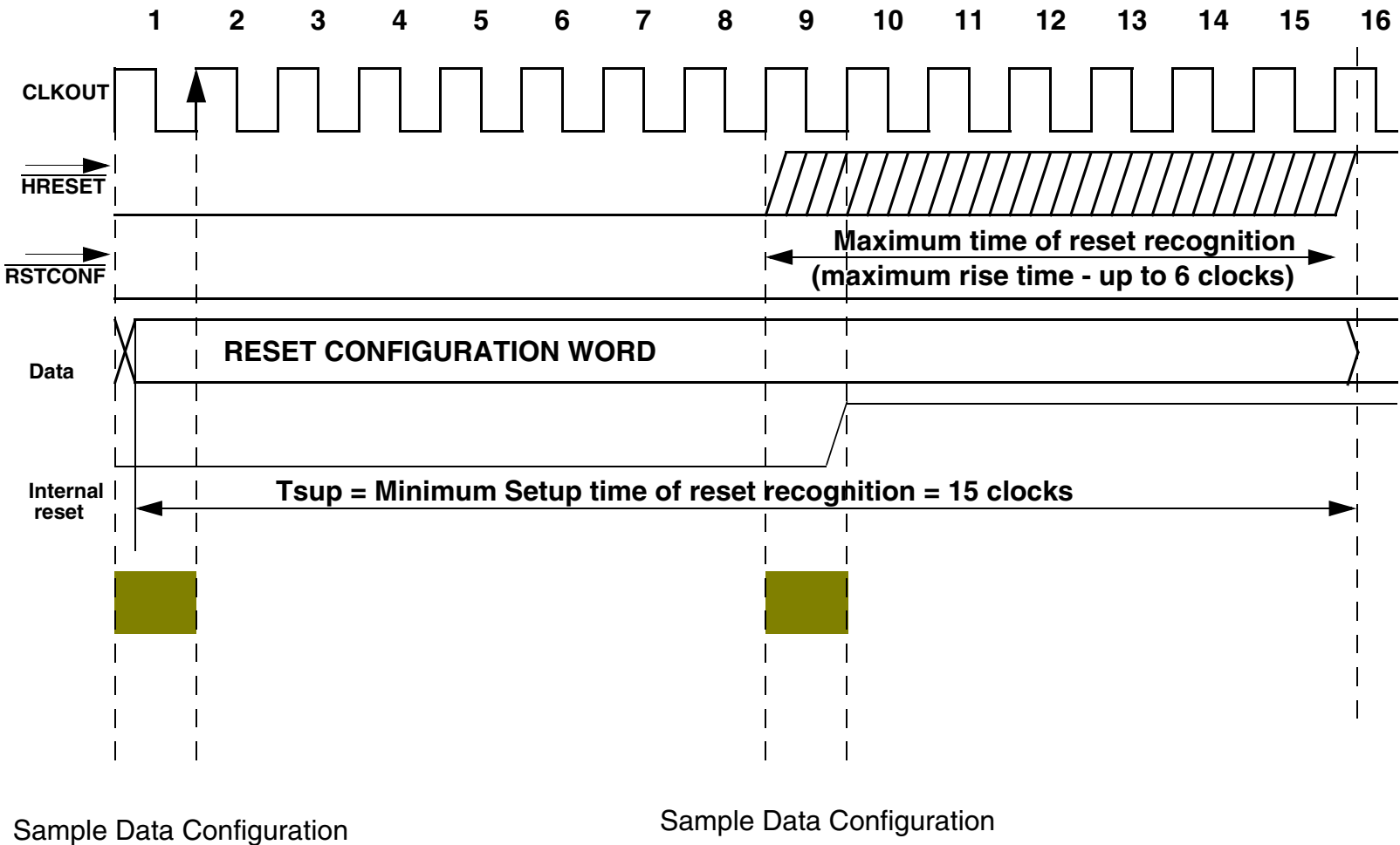
Figure 7-5 Reset Configuration Sampling Timing Requirements
