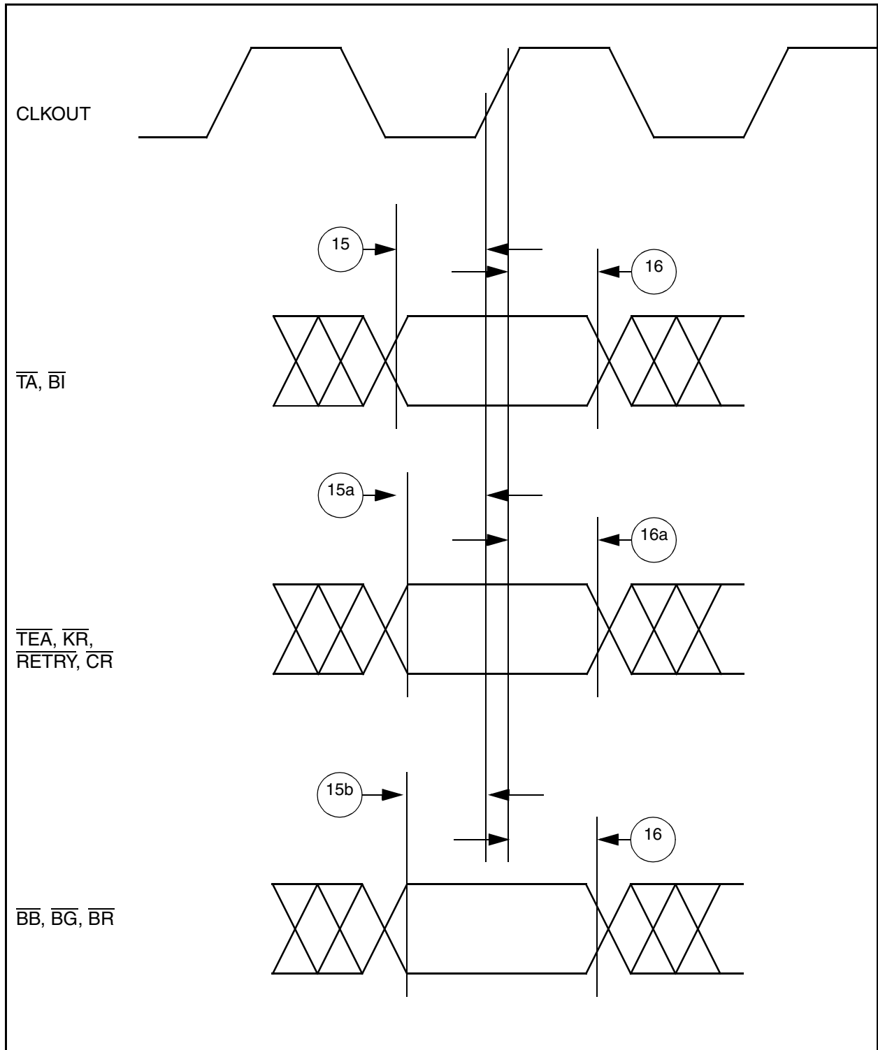
Figure G-5 Synchronous Input Signals Timing
