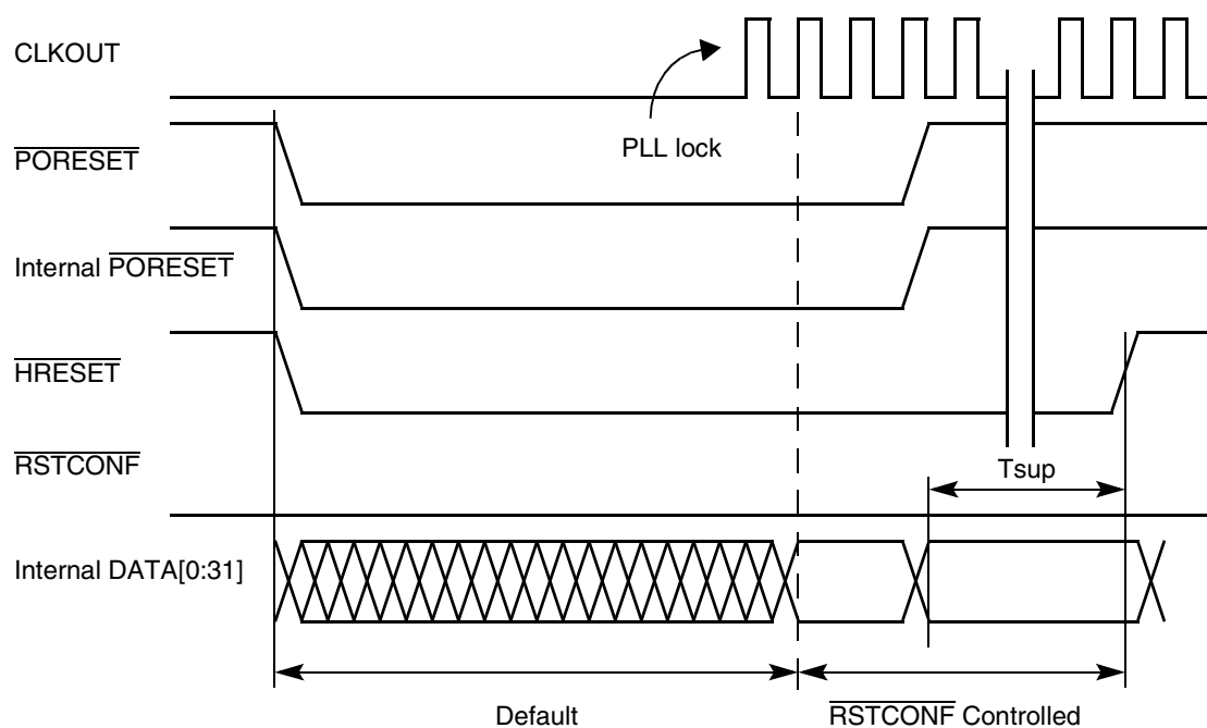
Figure 7-4 Reset Configuration Timing for PLL lock
