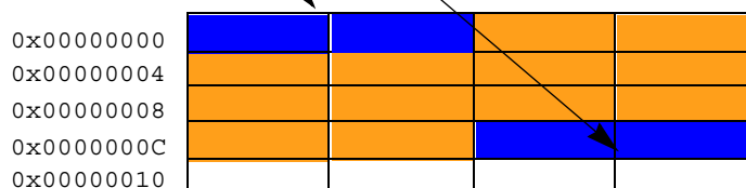
Figure 21-2 Partially Supported Watchpoint/Breakpoint Example
