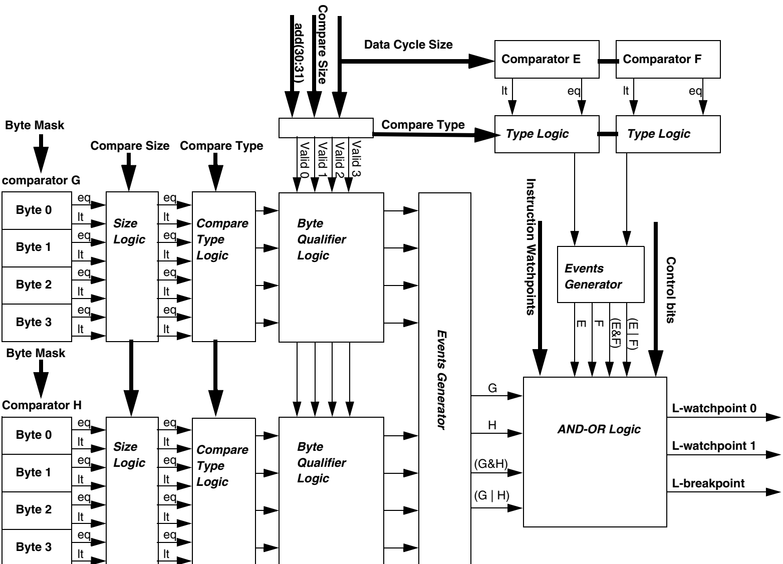
Figure 21-4 Load/Store Support General Structure
