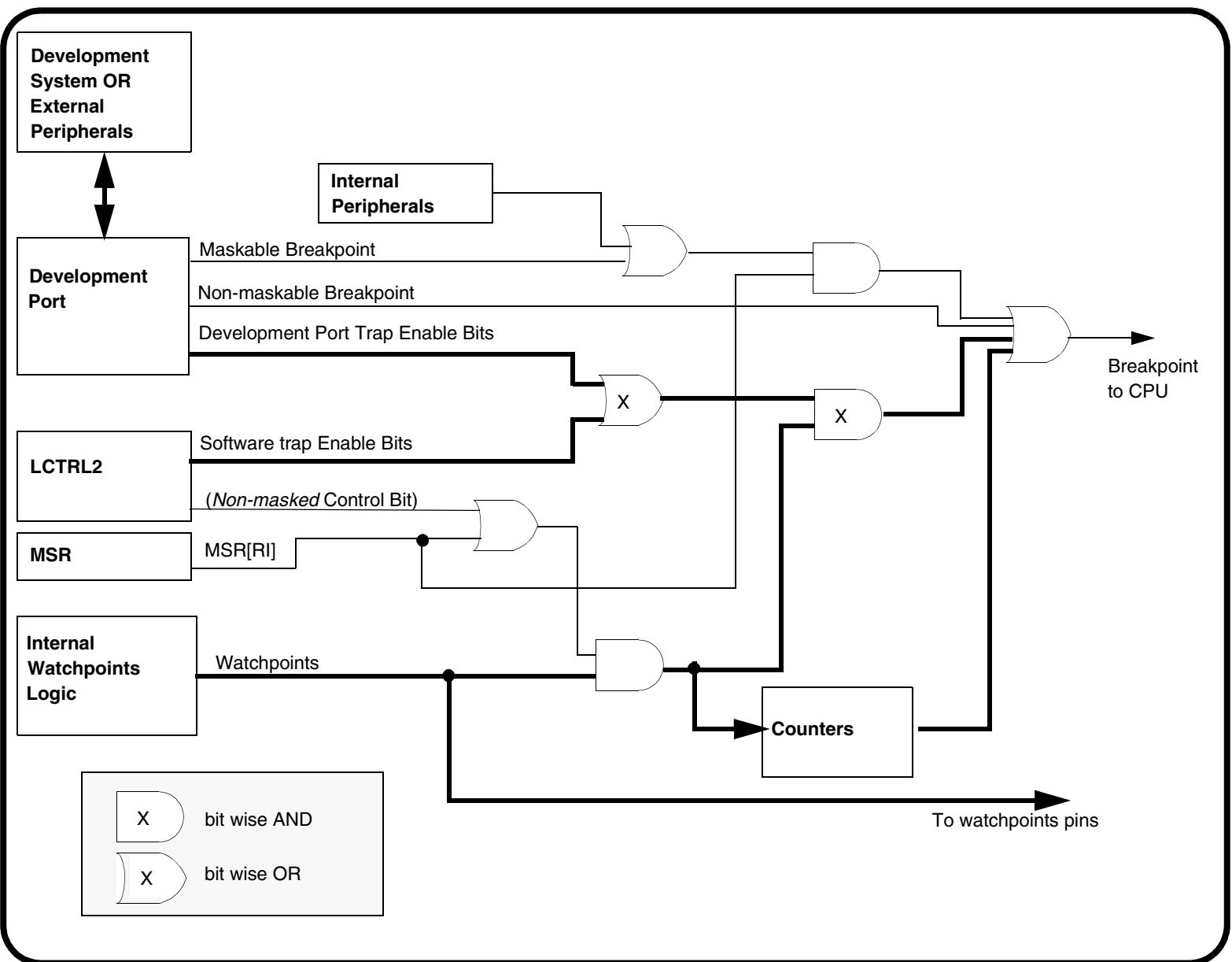
Figure 21-1 Watchpoints and Breakpoint Support in the CPU
