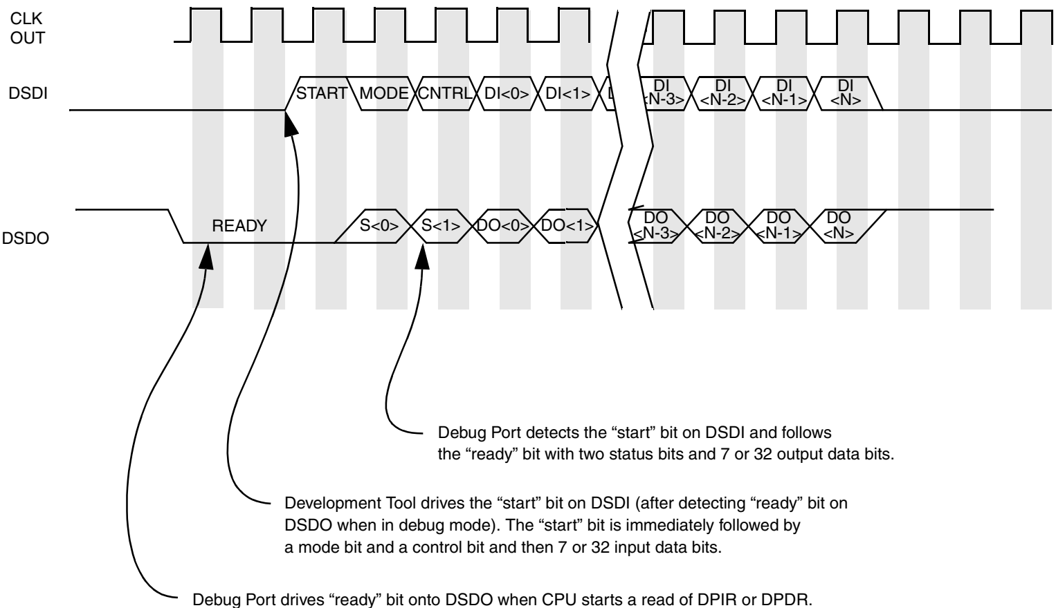
Figure 21-9 Synchronous Self Clock Serial Communication
