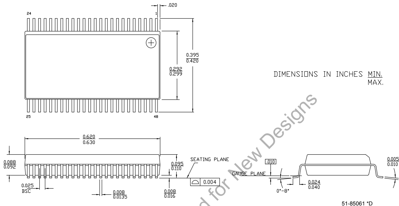
Figure 13. 48-Pin Shrunk Small Outline Package
