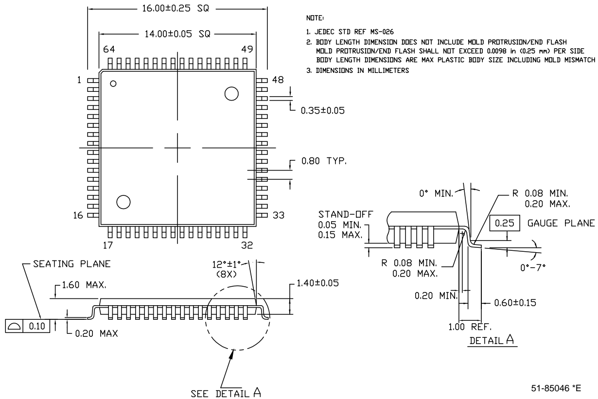
Figure 25. 64-Pin Thin Plastic Quad Flat Pack (14 × 14 × 1.4 mm), 51-85046
