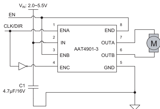
Figure 4: Full-Bridge Motor Driver Using AAT4901.
