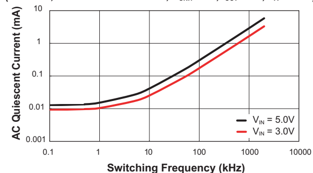
AAT4901-1 AC Quiescent Current vs. Switching Frequency
