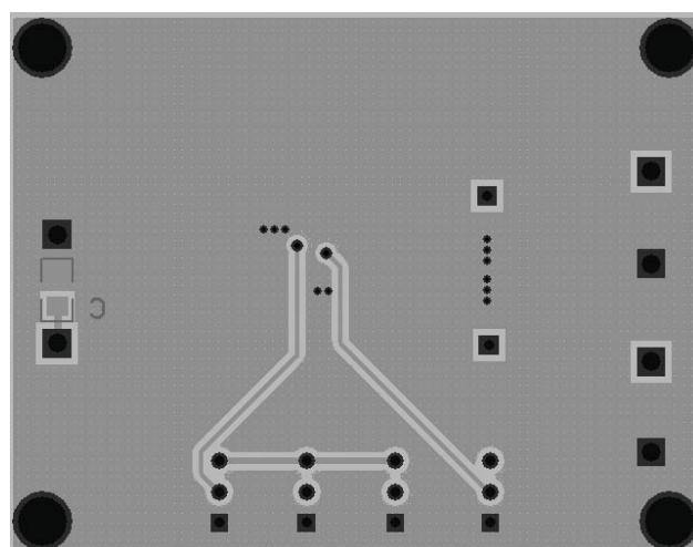
Figure 12: AAT4901 Evaluation Board Bottom Side Layout.
