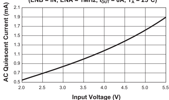
AAT4901-2 AC Quiescent Current vs. Input Voltage
