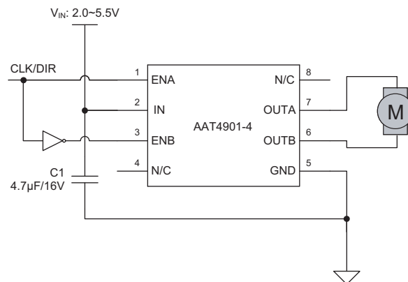
Figure 4: Full-Bridge Motor Driver Using AAT4901.
