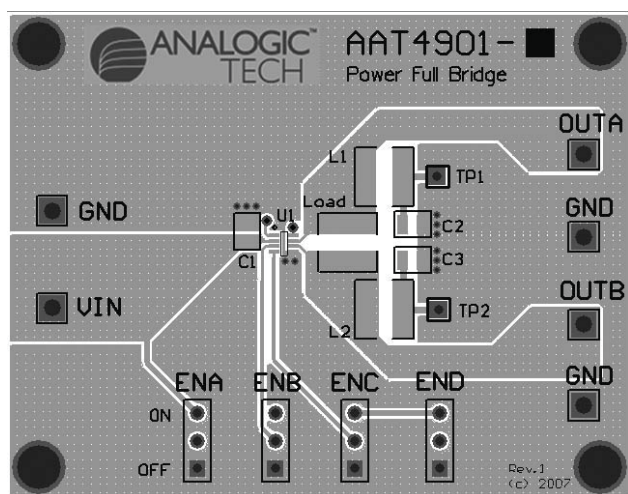
Figure 11: AAT4901 Evaluation Board Top Side Layout.
