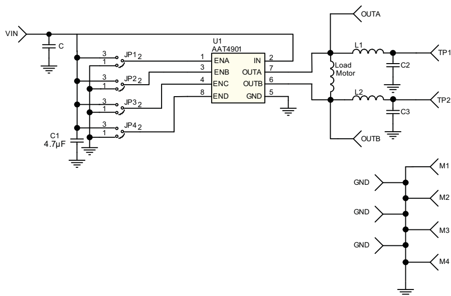
Figure 10: AAT4901 Evaluation Board Schematic.
