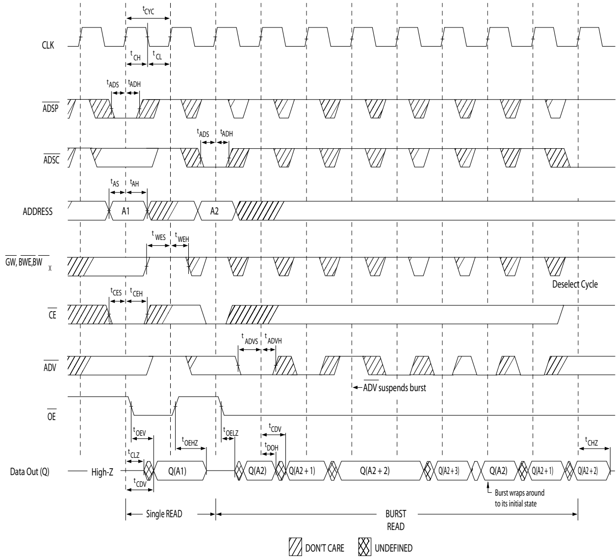
Figure 3. Read Cycle Timing [16]
