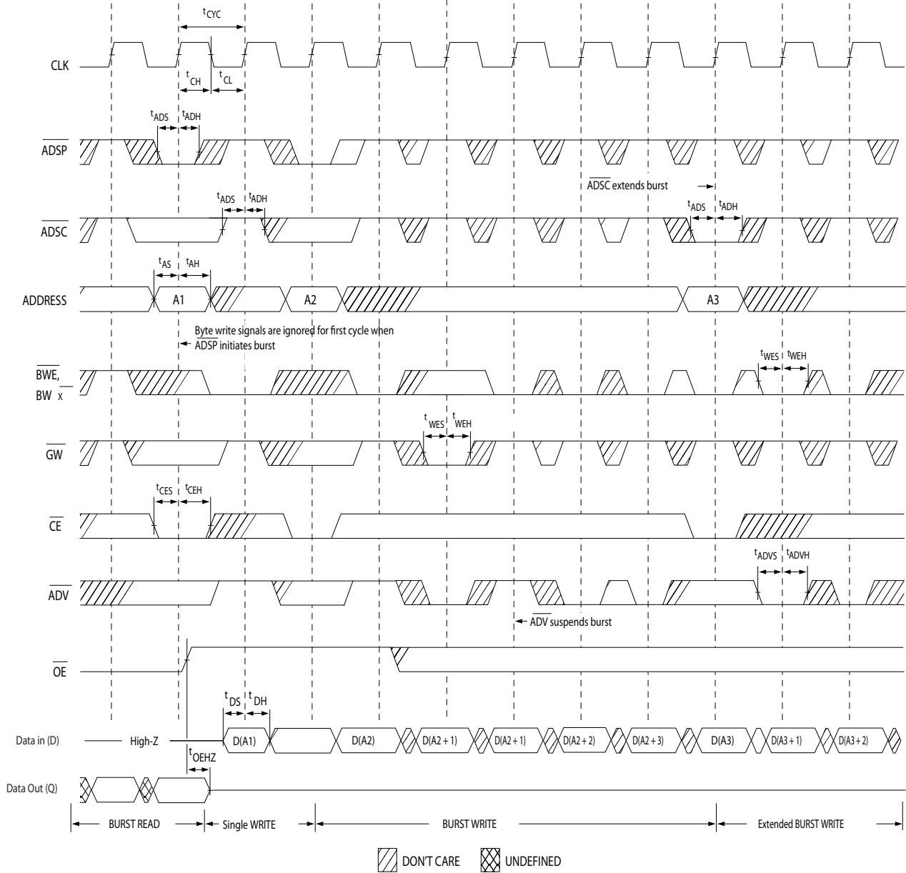
Figure 4. Write Cycle Timing [17, 18]
