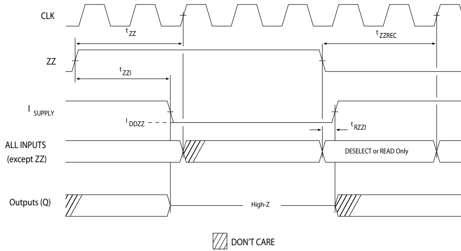
Figure 6. ZZ Mode Timing [22, 23]
