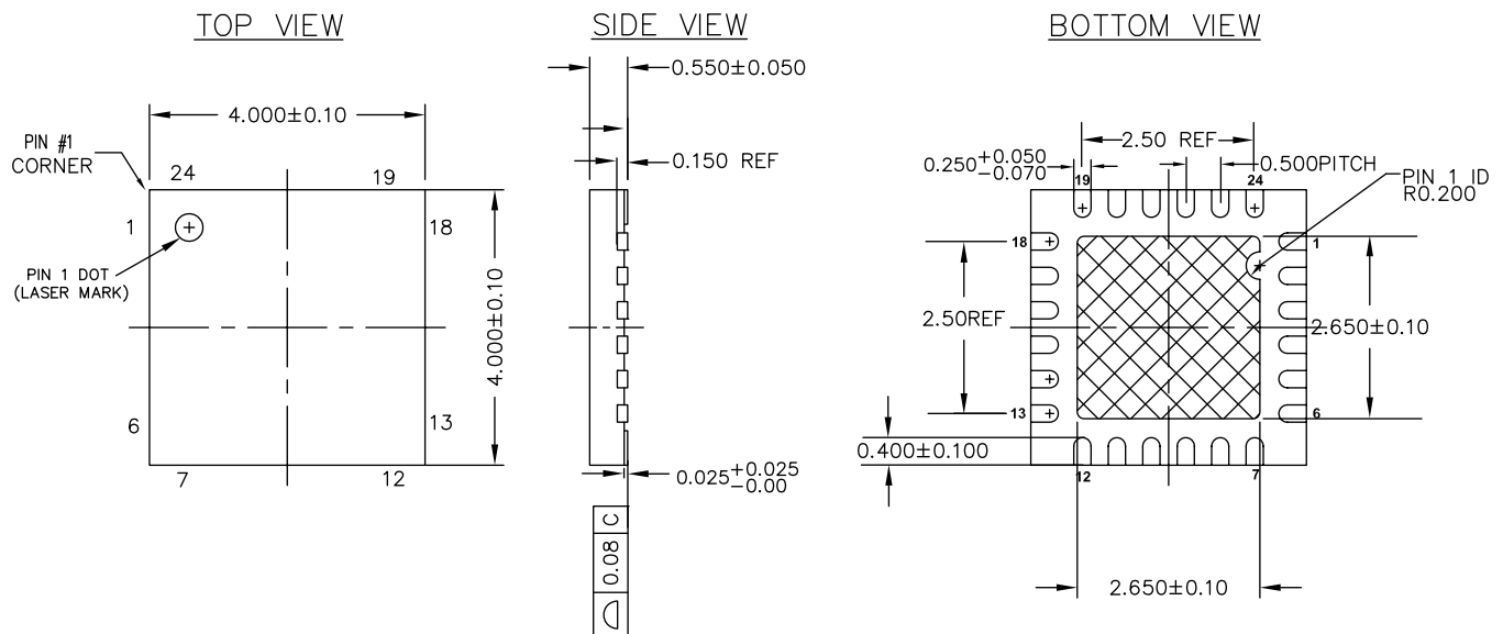
Figure 13. 24-Pin ( 4 \times 4 \times 0.55 mm) QFN
