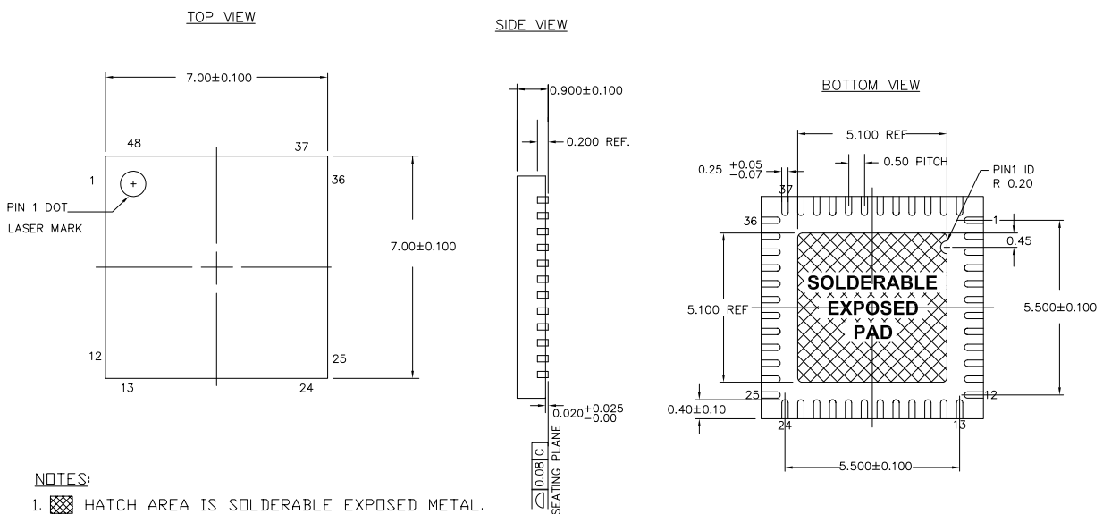
Figure 15. 48-Pin (7 × 7 × 1.0 mm) QFN
