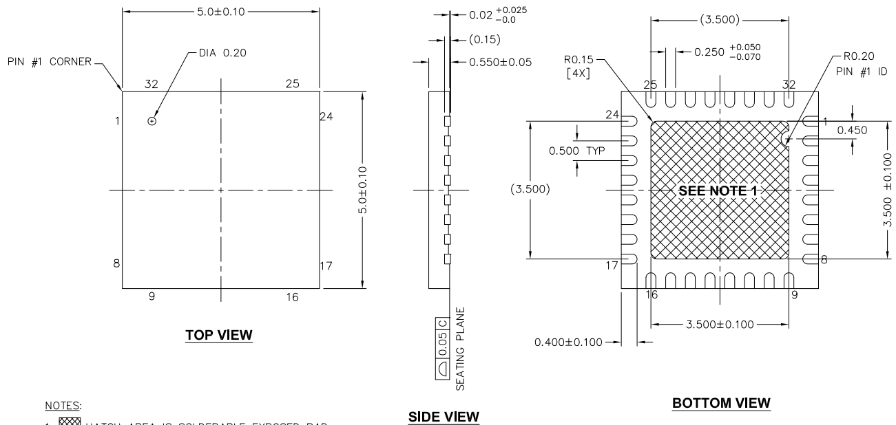
Figure 14. 32-Pin (5 × 5 × 0.55 mm) QFN
