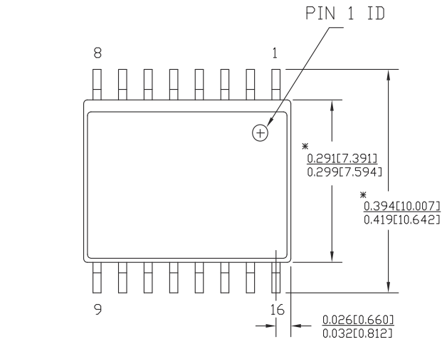
Figure 37. 16-pin SOIC (0.413 × 0.299 × 0.0932 Inches) Package Outline, 51-85022
