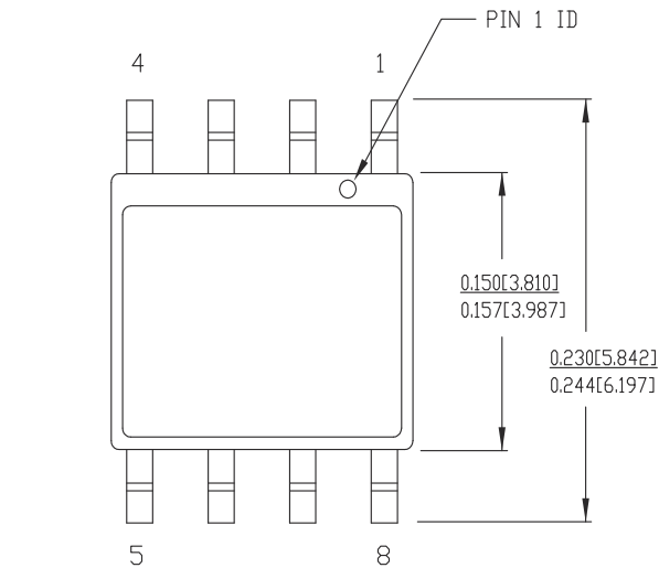
Figure 36. 8-pin SOIC (150 mils) Package Outline, 51-85066
