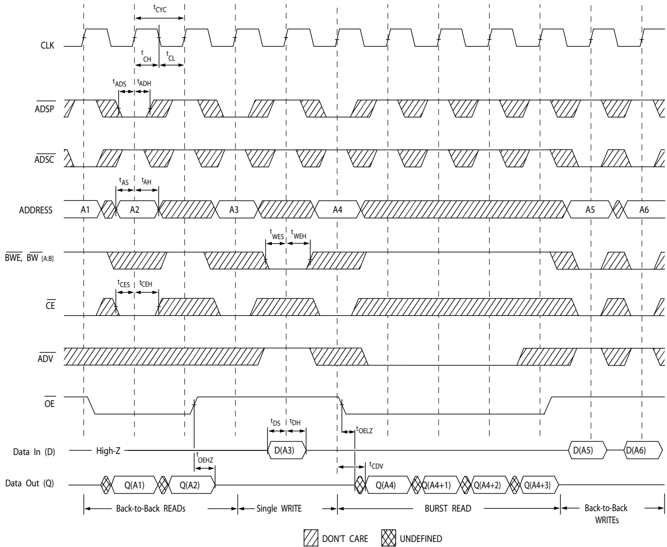
Figure 5. Read/Write Timing [19, 20, 21]
