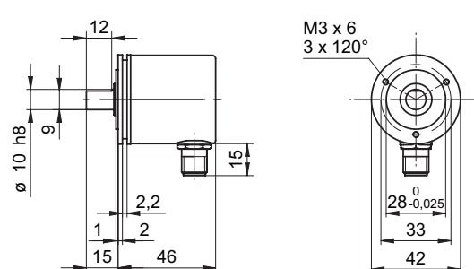
BMMV 42 SSI shaft 10 mm, connector M12 radial
