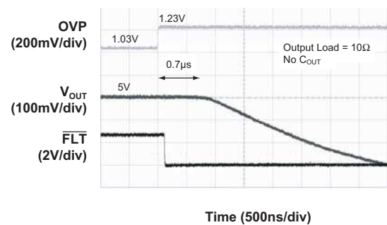
Figure 3: Typical Over-Voltage Response Time [zoom in].
