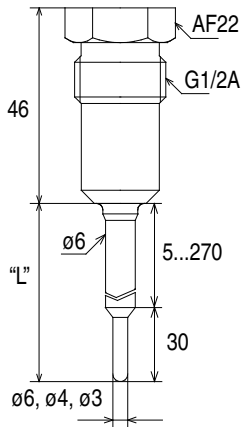
G1/2A male nipple, hygienic (welding part PM020)
