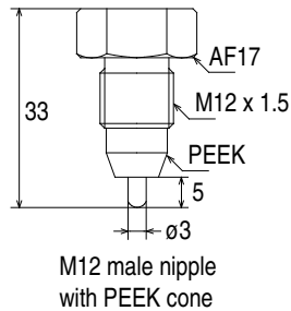
M12 male nipple, hygienic (welding part PM031)
