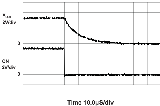
AAT4616IPS-1 and AAT4616IGV-1 Turn-Off ( R_L = 10\Omega ; C_L = 0.47\mu\text{F} )
