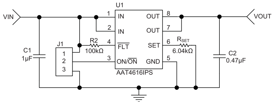
Figure 2: AAT4616IPS Evaluation Board Schematic
