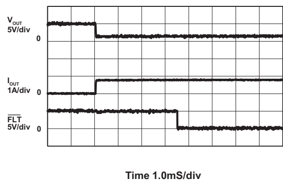
Fault Masking Time V_{\text{IN}} = 5\text{V}
