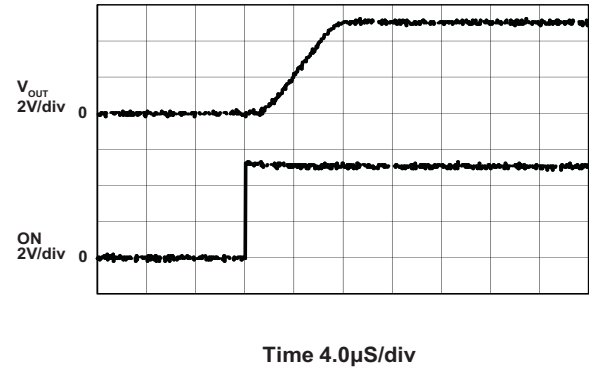
AAT4616IPS-1 and AAT4616IGV-1 Turn-On ( R_L = 10\Omega ; C_L = 0.47\mu\text{F} )
