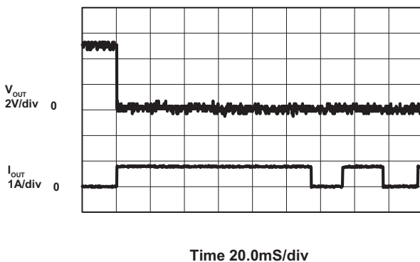
Output Short Response V_{\text{IN}} = 5\text{V}
