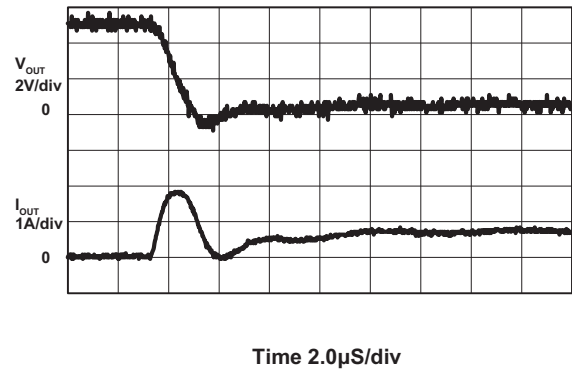
Short Circuit Through 0.3\Omega V_{\text{IN}} = 5\text{V}
