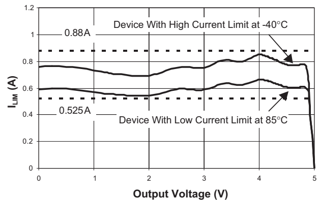
Figure 1: Current Limit Using 10.5k\Omega .
