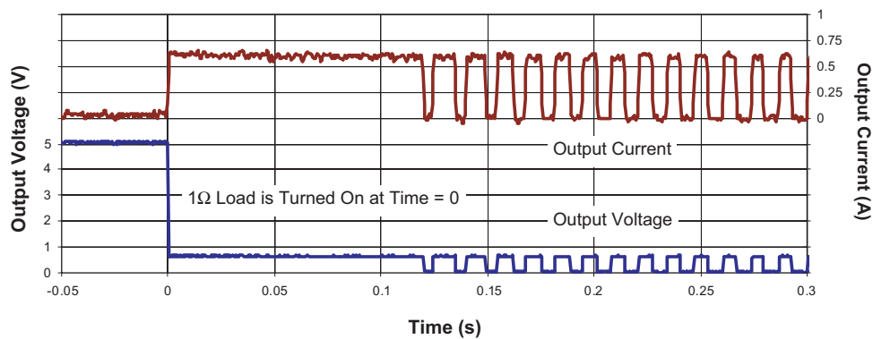
Figure 2: Overload Operation.
