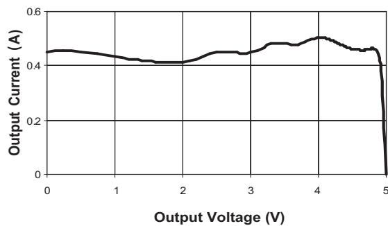
Output Current vs. Output Voltage ( R_{SET} = 16k\Omega )
