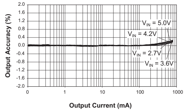
DC Regulation
