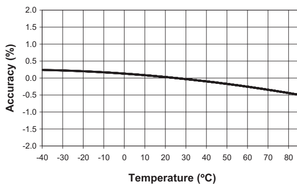
Output Voltage Accuracy vs. Temperature
