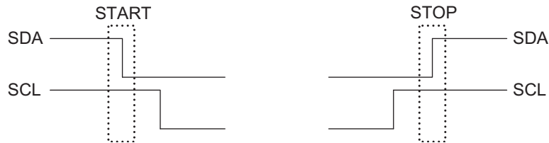
Figure 2: I 2 C Start and Stop Conditions.
