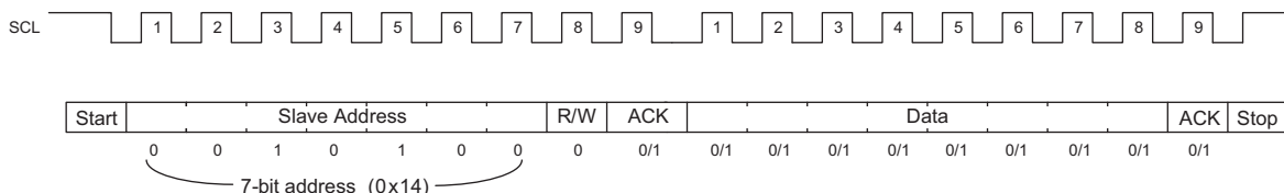
Figure 5: I 2 C SCL, SDA Transfer Protocol Example; 7-bit Slave Address (A6-A0 = 0x14), 1-bit Read/Write (R/W = 0), 1-bit Acknowledge (ACK), 8-bit Data (D7-D0), 1-bit Acknowledge (ACK).
