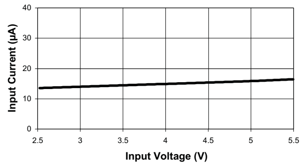
Quiescent Current
