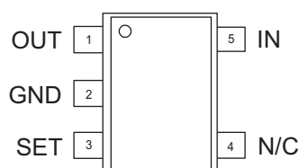
SOT23-5 (Top View)
