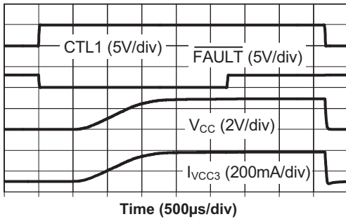
Turn-On/Off Response (10 \Omega , 1 \mu\text{F} Load)
